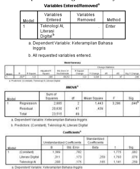
Figure 6. Multiple Linear Regression Analysis
